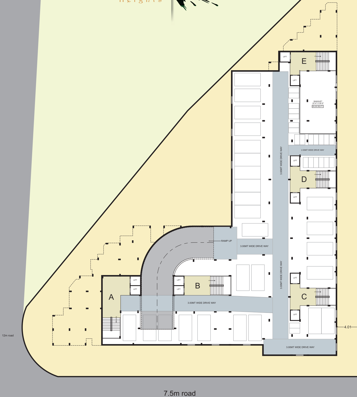
CELLAR LAY - OUT PLAN
